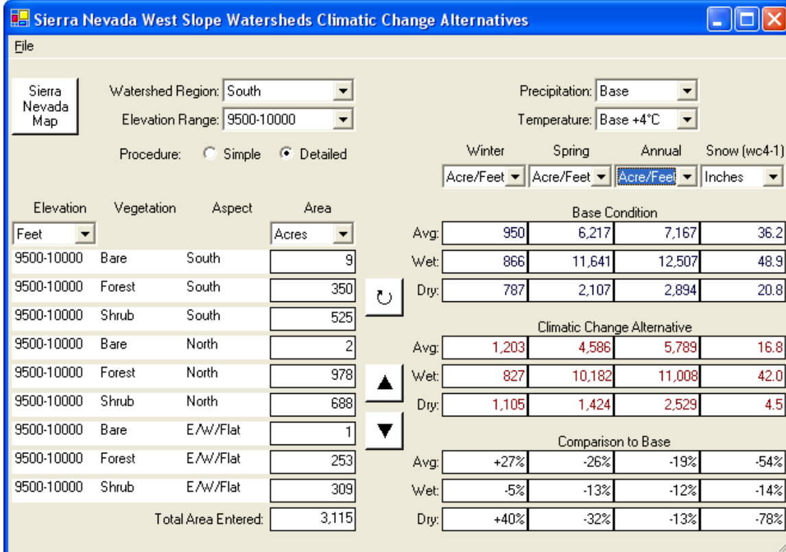
Bear Creek: 9500-10000 feet elevation profile, inches and acre-feet
