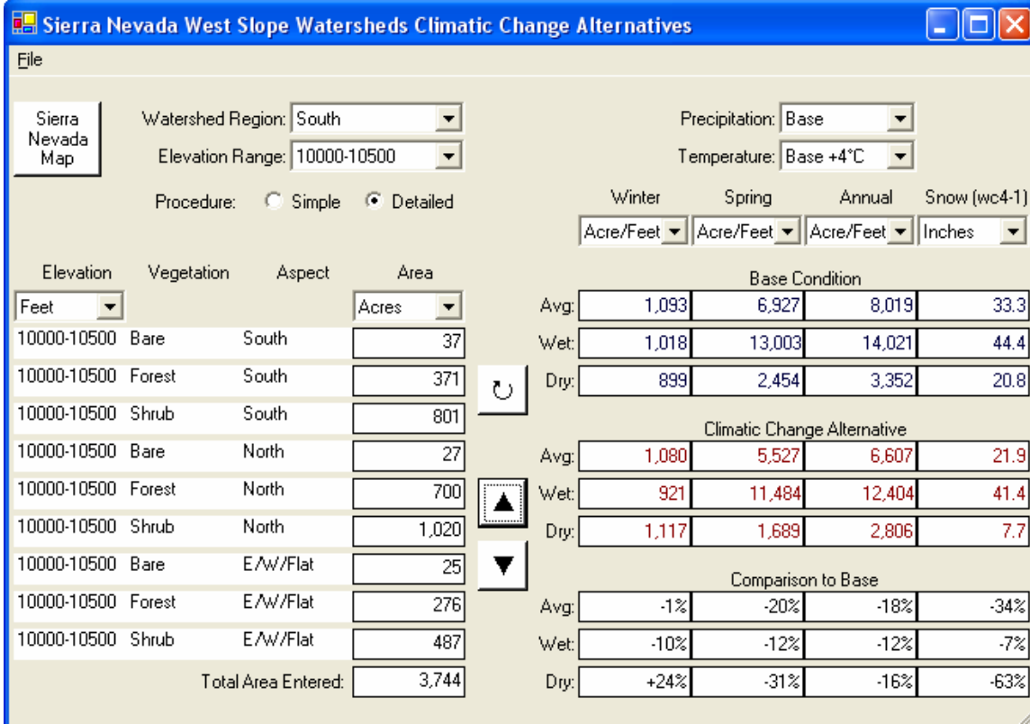
Bear Creek: 10000-10500 feet elevation profile, inches and acre-feet
