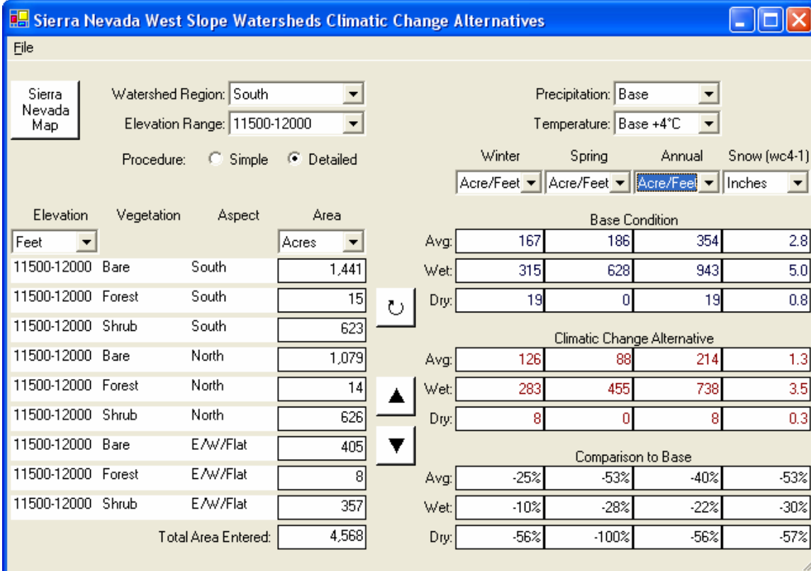
Bear Creek: 11500-12000 feet elevation profile, inches and acre-feet
