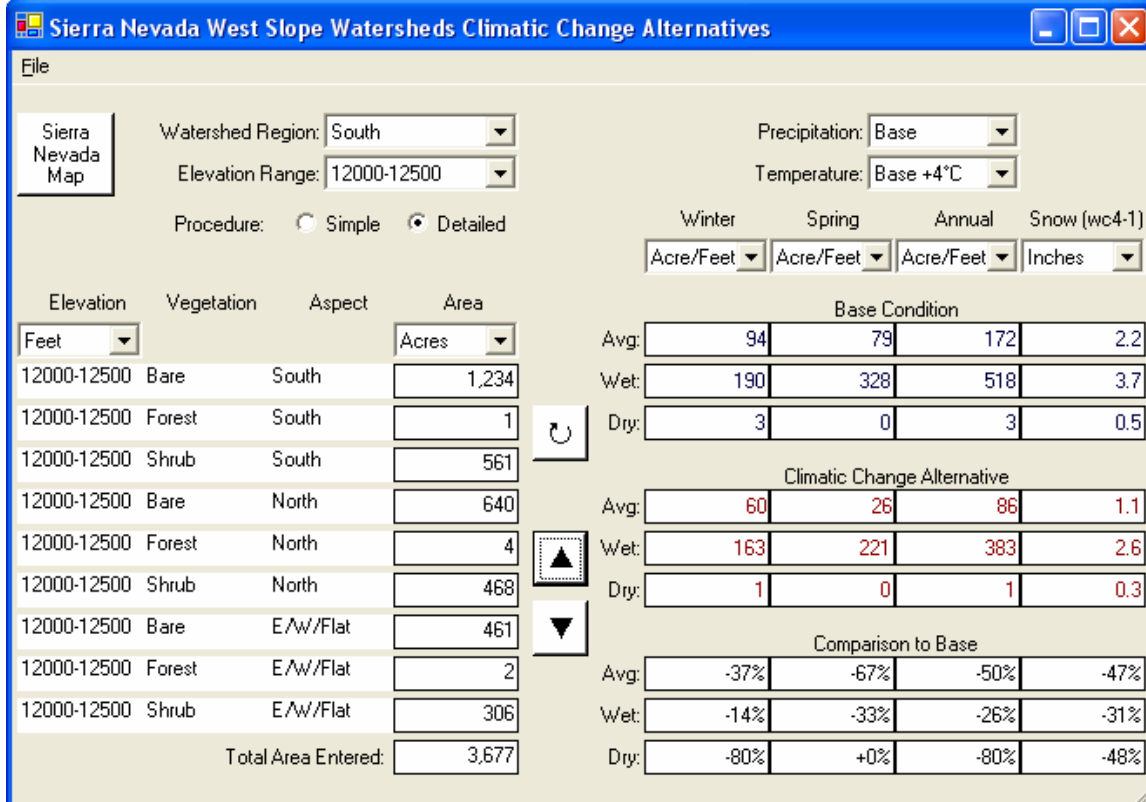
Bear Creek: 12000-12500 feet elevation profile, inches and acre-feet
