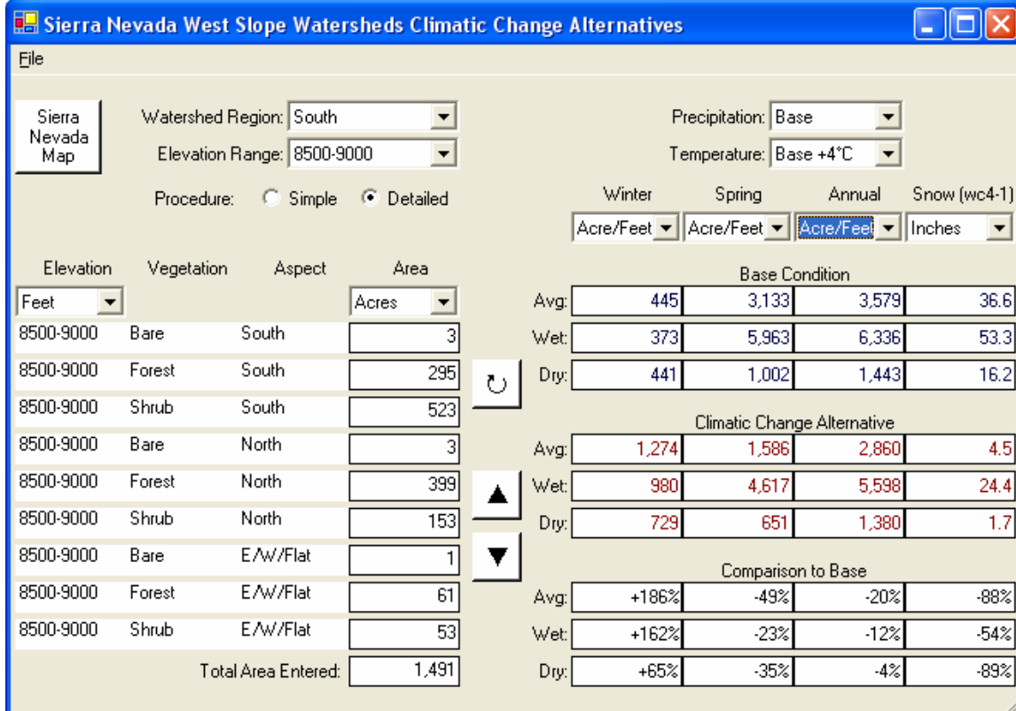
Bear Creek: 8500-9000 feet elevation profile, inches and acre-feet
