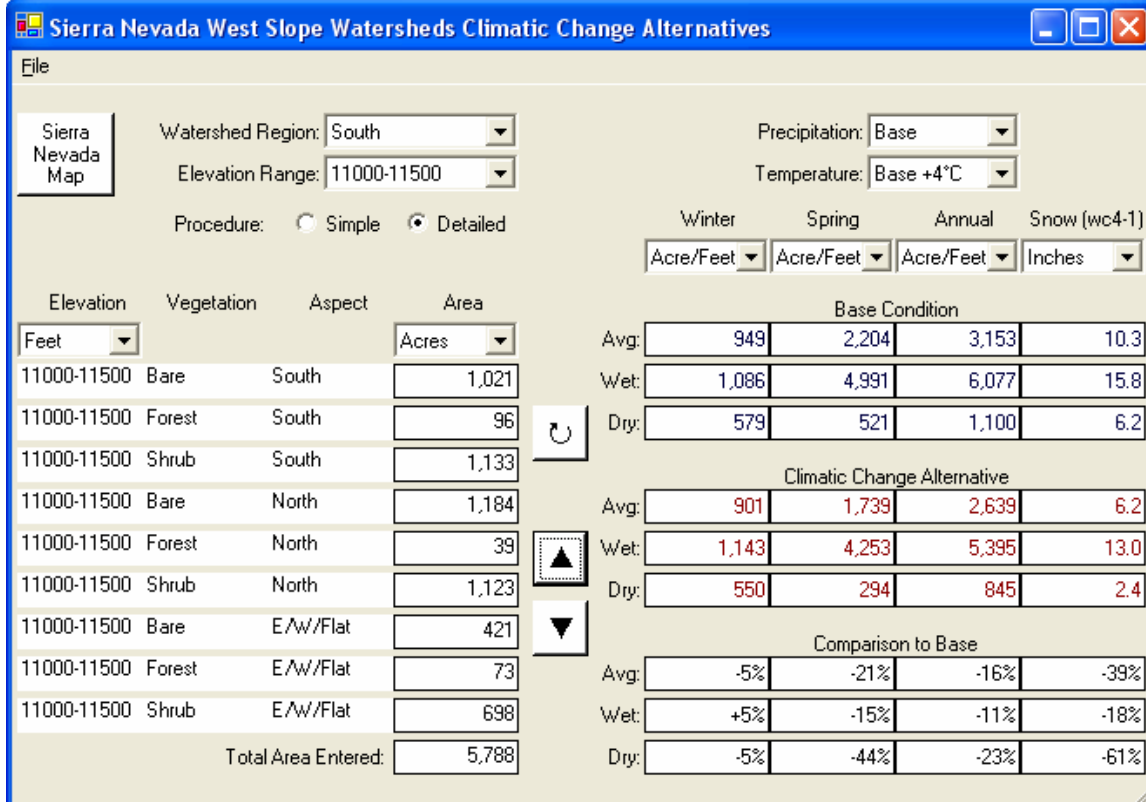
Bear Creek: 711000-11500 feet elevation profile, inches and acre-feet
